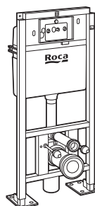
Duplo WC Freestanding
